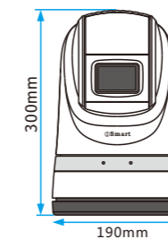
With Damper
